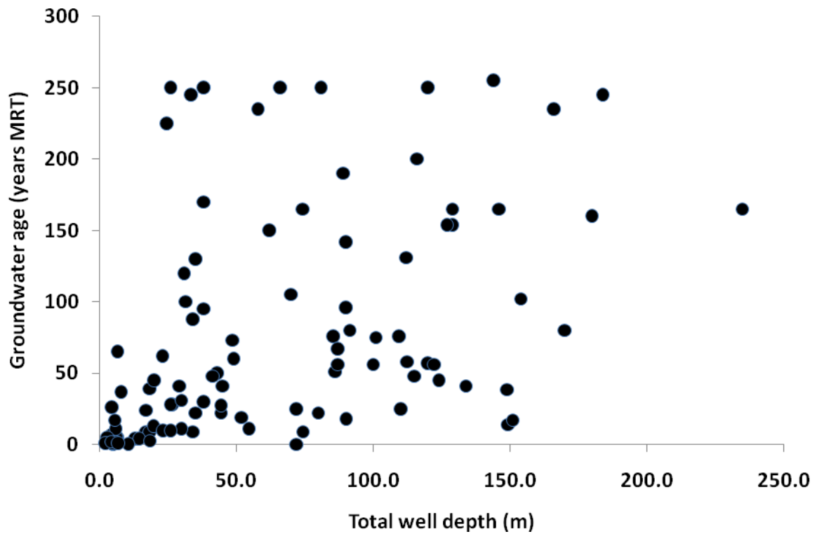
Figure 8: Groundwater age versus well depth for the Healthy Rivers area
