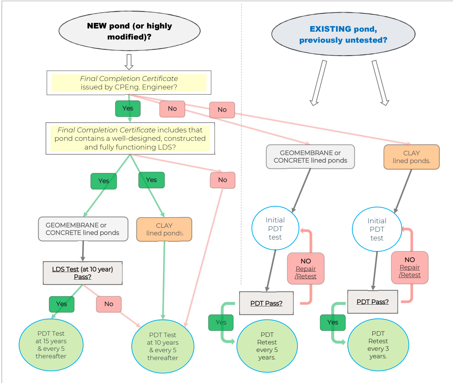
Figure 1: PDT Testing Frequency Flowchart for Effluent Ponds
