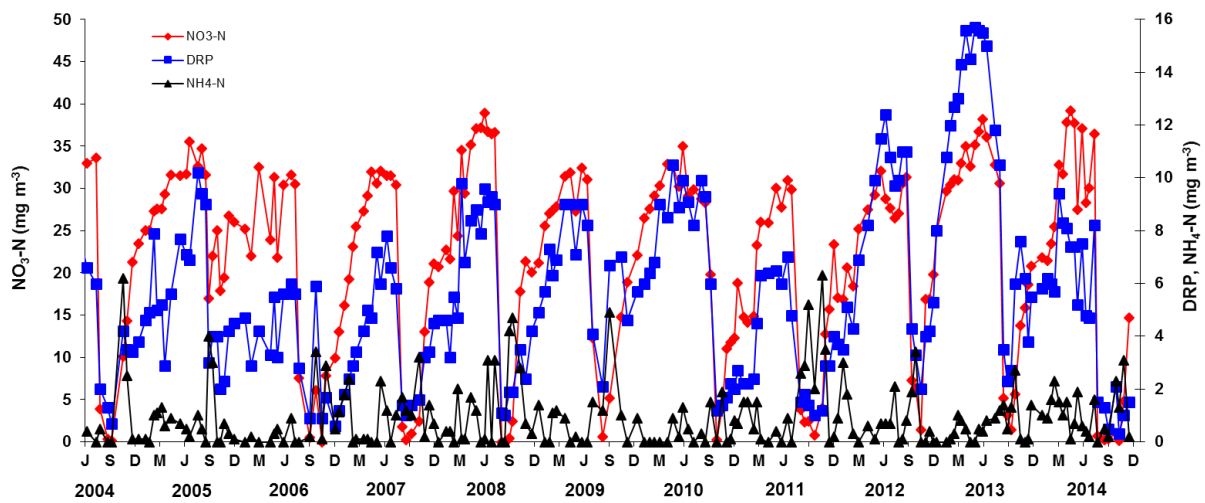
Figure 19: Time series bottom water nutrient data. DRP, NO 3 -N and NH 4 -N concentrations in the bottom waters (150 m depth) of Lake Taupo since winter mixing of 2004. (Starting tick “J” = June with 3-monthly increments).
