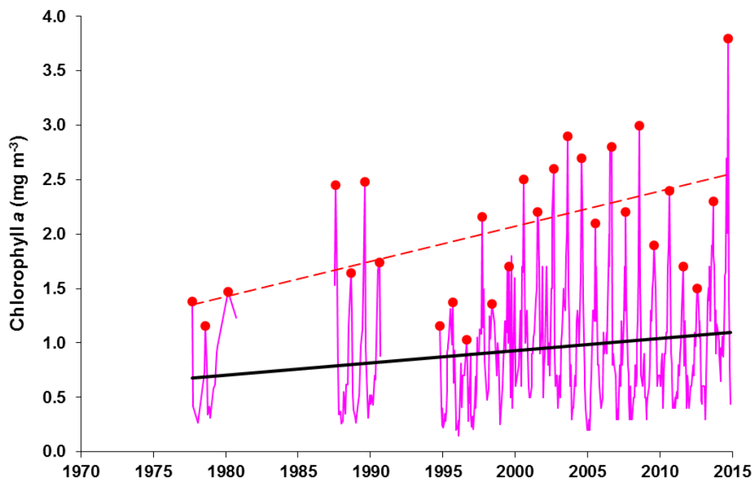
Figure 14: Time-series chlorophyll a concentrations from the 10-m tube samples since 1977. Average concentrations increased at a rate of 0.0114 \pm 0.006 \text{ mg m}^{-3} \text{ y}^{-1} ( P < 0.0005 , r^2 = 0.03 , n = 407 ) while winter maximum concentrations (red dots) increased at a rate of 0.032 \pm 0.022 \text{ mg m}^{-3} \text{ y}^{-1} ( P < 0.005 , r^2 = 0.268 , n = 28 ). Data prior to 1994 are unpublished results collected by the Taupo Research Laboratory, DSIR, using the same 10 m integrated-tube sampling technique and analytical method.
