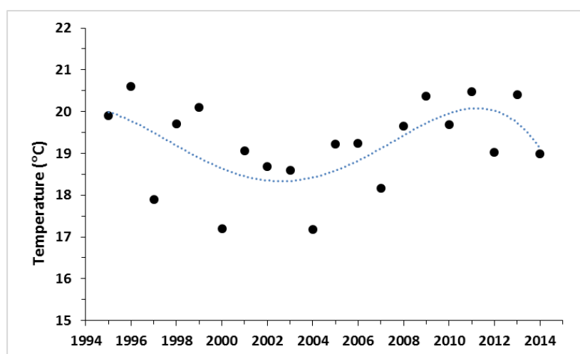
Figure 3: Maximum 20 m temperatures in summer. The trend line is a 4th order polynomial indicating a pattern of warmer and cooler summers.
