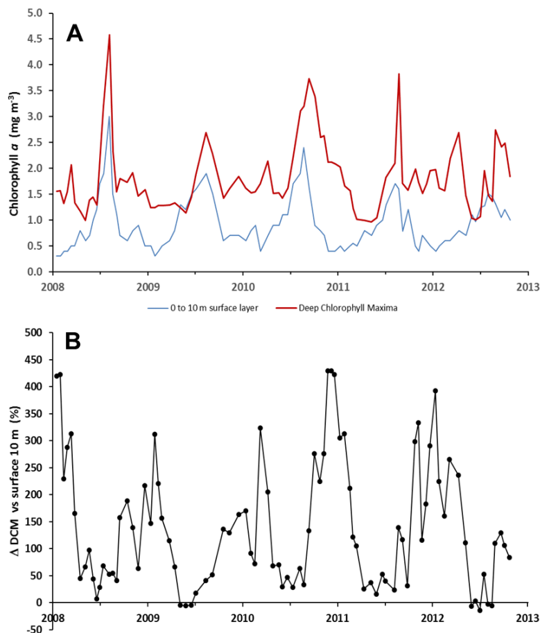
Figure 16: DCM data from 2008 to 2012. A) Comparison of chlorophyll a concentrations in the 0 to 10 m layer and the chlorophyll a in the DCM layer calculated from calibrated chlorophyll fluorescence profiles, and B) The difference between the DCM and the 0 to 10 m depth layer, as a percentage of the surface concentration.
