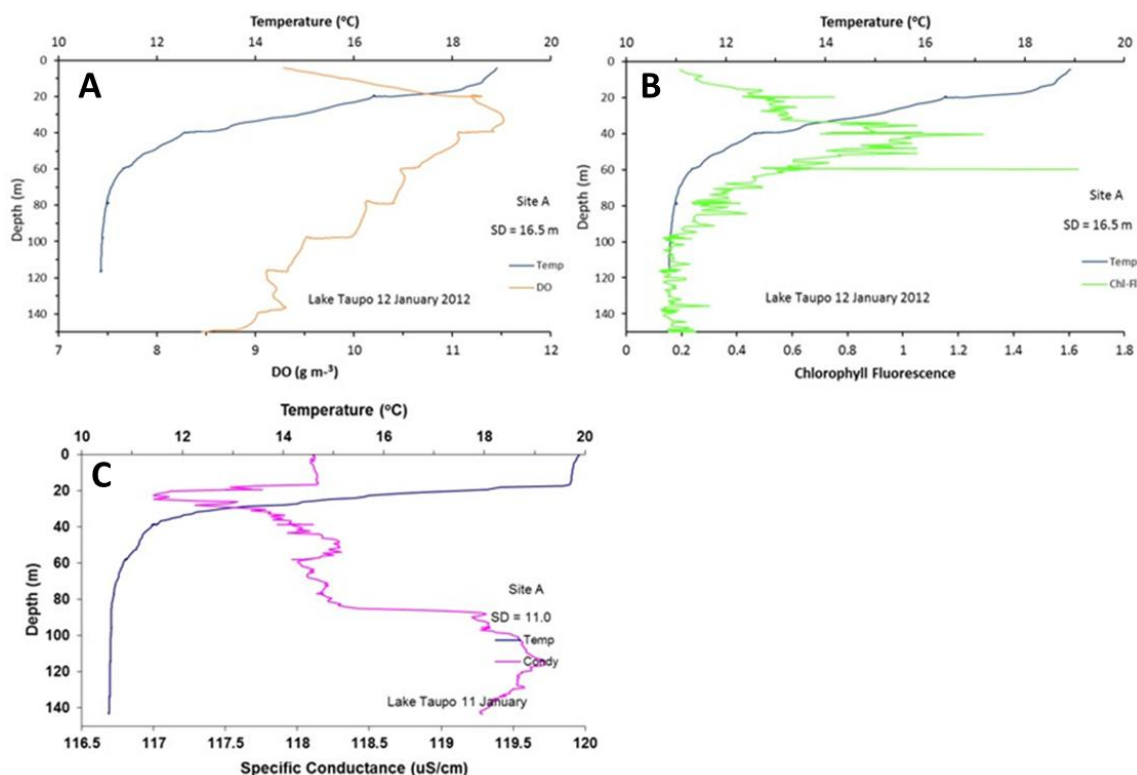
Figure 6: Lake Taupo CTD-O profile examples. A) Dissolved oxygen, and B) Chlorophyll fluorescence in January 2012 and C) conductivity in January 2011 relative to temperature and depth.
