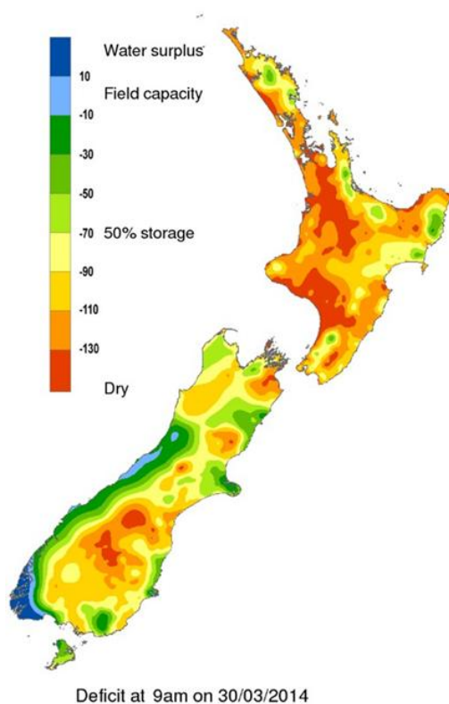
Figure 4: NIWA soil moisture anomaly map for March 2014 showing the extent of the 'drought'. The whole of the Lake Taupo catchment was affected for at least three months.
