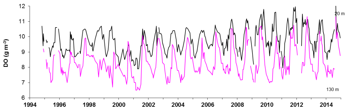
Figure 5: Time-series dissolved oxygen data. Time-series dissolved oxygen data from 20 m (black line) and 130 m (pink line) depths. Mixing and reoxygenation occurred where the 2 lines in the temperature data (Figure 2) meet each winter. However, where temperature data indicate incomplete mixing there is incomplete reoxygenation of the hypolimnion. Date ticks are 1 January in each year.
