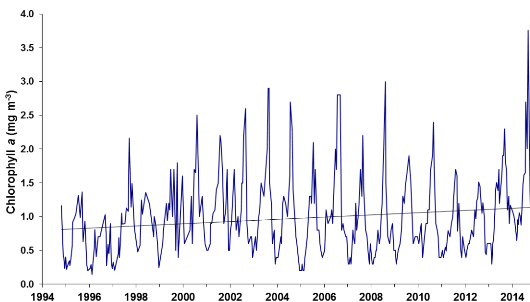
Figure 12: Time-series chlorophyll a concentrations in the upper 10 m of Lake Taupo. The solid regression line represents a statistically significant increase in the mean chlorophyll a concentrations of 0.016 \pm 0.010 \text{ mg m}^{-3} \text{ y}^{-1} ( P = 0.0017 , r^2 = 0.028 , n = 352 ). Date ticks are 1 January in each year.
