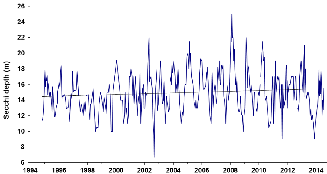
Figure 9: Water clarity as measured by Secchi depth. Time-series Secchi depth data for the present monitoring programme since 1994. Trend line equation 0.059 \pm 0.079 \text{ m y}^{-1} ( P = 0.154 , r^2 = 0.11 n = 350 ).
