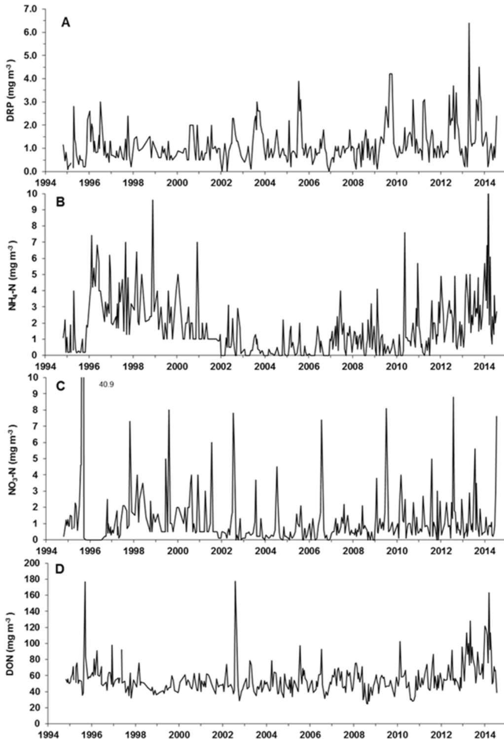
Figure 18: Time series nutrient data in Lake Taupo. Time series data from the top 10 m of the water column in Lake Taupo for (A) dissolved reactive phosphorus (DRP), (B) ammoniacal nitrogen ( \text{NH}_4\text{-N} ), (C) nitrate + nitrite nitrogen ( \text{NO}_3\text{-N} ), and (D) dissolved organic nitrogen (DON). Broken line indicates the long term minimum DON concentration of 29 \text{ mg m}^{-3} , which may be mostly refractory organic material. Date ticks are 1 January in each year.
