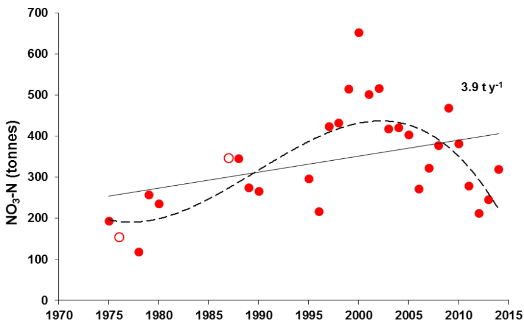
Figure 21: Total mass of \text{NO}_3\text{-N} in the hypolimnion of Lake Taupo in autumn before winter mixing. The linear regression (solid line) indicates a weakly significant increase of 3.9 \text{ t y}^{-1} ( P = 0.06 , r^2 = 0.13 , n = 27 ). Temporal changes in the data are better described by a 3 rd order polynomial (dashed line) ( r^2 = 0.519 ) which accommodates a rise and fall in the data over the monitoring period since 1974. Open circle data were excluded from regression as time periods and sampled depths were not the same as used for the other data. Date ticks are 1 January in each year.
