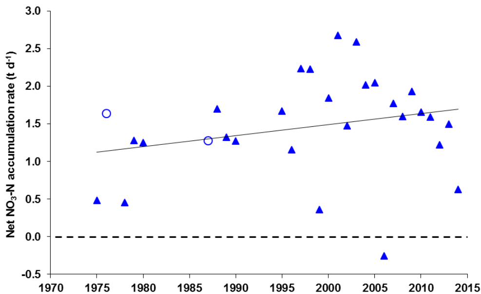
Figure 23: Net Hypolimnetic NO 3 -N accumulation rates. Net NO 3 -N accumulation rates (t d -1 ) in the hypolimnion below 70 m. The regression line shows an increase in the net accumulation rate of 0.015 \pm 0.024 t d -1 ( P = 0.22 , r^2 = 0.059 , n = 27 ). Open circle data were not included in the regression analysis (see text). Note that the Y-axis extends to -0.5 t d -1 for the 2006 data point. Date ticks are 1 January in each year.
