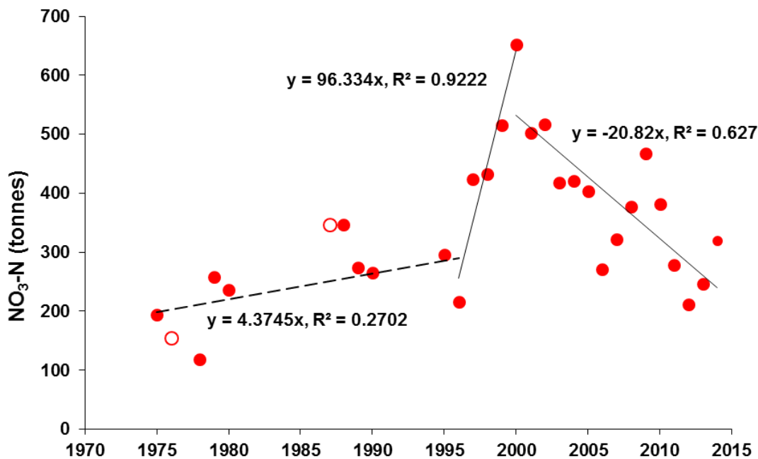
Figure 22: Changes in nitrate (NO 3 -N) accumulation in the hypolimnion of Lake Taupo. The last regression line shows that in the last 15 years, NO 3 -N mass has decreased at a significant average rate of around 20.8 t y -1 (P<001, r 2 = 0.63, n = 15) and is now comparable with the estimated mass present in the late 1970s and early 1980s.
