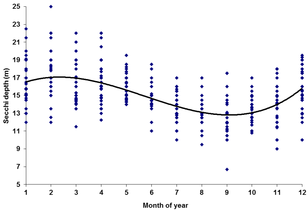
Figure 10: Seasonal cycle of water clarity (1994 -2014). The annual pattern of all water clarity data has a seasonal cycle with minimum clarity occurring usually in September.
