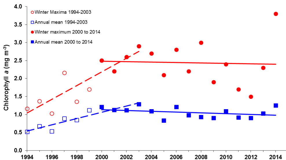
Figure 13: Annual mean and maximum chlorophyll a concentrations. Annual mean and winter maximum chlorophyll a concentrations from the 10-m tube samples since 1994. Regression lines indicate significant ( P < 0.001 ) trends of increase between 1994 and 2003 (broken lines) but non-significant ( P = 0.22 ; maximum and P = 0.87 ; mean) trends of decrease from 2000 to 2014 (solid lines). These regressions overlap between 2000 and 2003. Regression slopes are given in the text. Date ticks are 1 January in each year.
