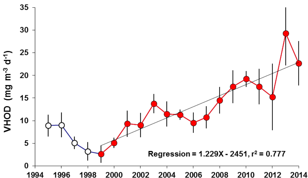
Figure 8: Time-series VHOD data. Time-series of VHOD rates since 1994-5. The low VHOD in 1997-2000 (following the 1995/96 eruptions of Mount Ruapehu) correlates with a shift in algal dominance from diatoms to colonial greens ( Botryococcus braunii ). The regression through the solid (red) dots ( P < 0.0001 , r^2 = 0.78 , n = 16 ), only refers to the change in VHOD since 1998/99, the year when the VHOD rate during the monitoring programme was lowest, and the last year in which diatoms were not dominant. Bars are SD.
