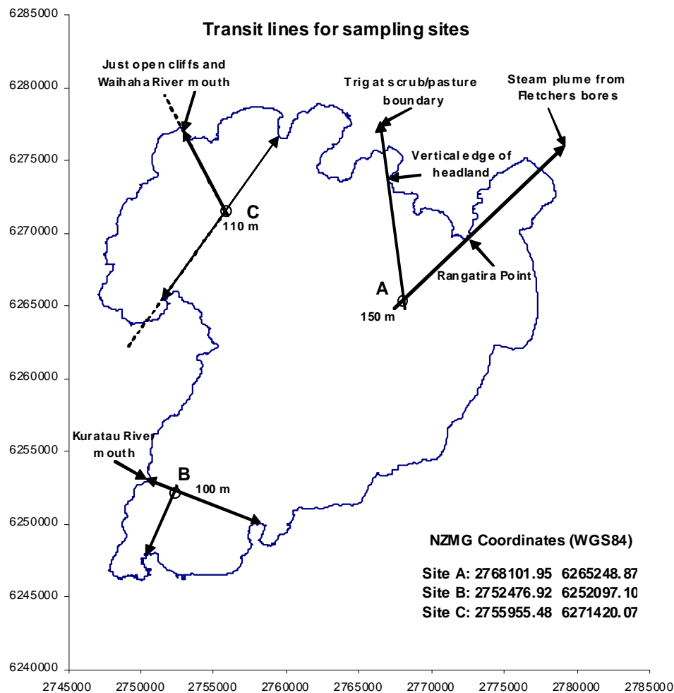
Figure 25: Site map of Lake Taupo. Site map of Lake Taupo showing location of the routine monitoring site at mid lake (A). Two additional sites at Kuratau Basin (B) and the Western Bays (C) were sampled between January 2002 and December 2004 inclusive. Data from those sites have been retained with the Site A data presented in the appendices. Map coordinates are in NZ Map Grid with WGS84 correction. Lat. Long WGS 84 corrected co-ordinates of "Site A" are 38° 46'.810 S; 175° 58'.440 E.
