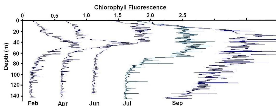
Figure 17: Fluorescence profiles in Lake Taupo. Selected sequential chlorophyll fluorescence profiles during 2010 showing the progression from a deep chlorophyll maxima in summer to its disappearance and sedimentation of algal matter during the winter bloom. Each profile is offset to the right by successive 0.5 chlorophyll fluorescence units for clarity.
