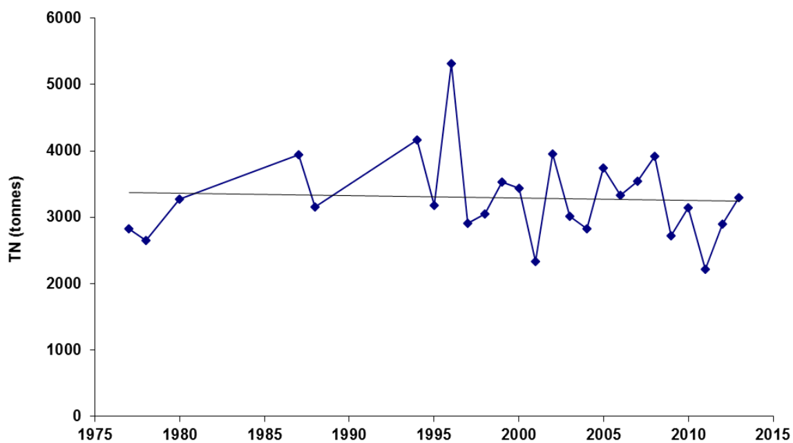
Figure 24: Estimates of the mass of total nitrogen (TN) in Lake Taupo. Although there was an average decrease of about 3.5 \text{ t y}^{-1} from 1975 to 2014, this apparent trend in the data is not statistically significant ( P = 0.79 , n=25 , r^2 = 0.003 ). The mean was 3294 t. Date ticks are 1 January in each year.
